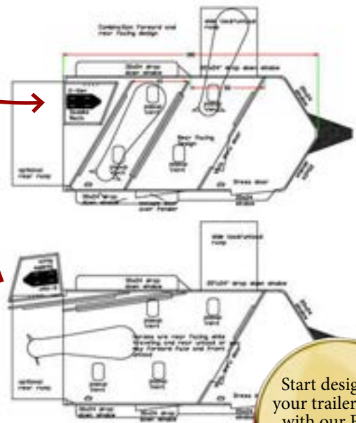
Reverse Safetack Slant Load with Side Ramp
