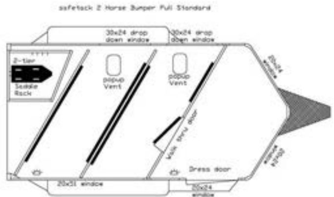
Forward Facing Safetack Slant Load
