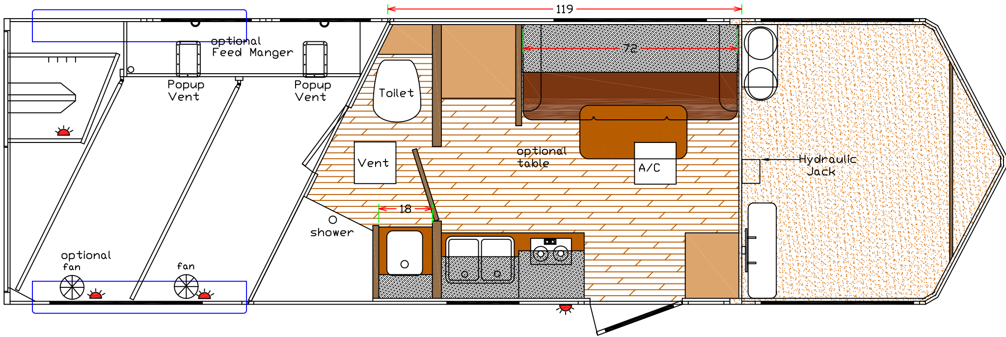
Safetack Rawhide EX package, shown in 2H Version, available in 3H and 4H
